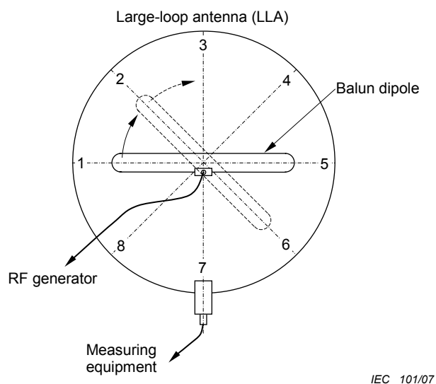
Figure C.7 – The eight positions of the balun-dipole during validation of the large-loop antenna
