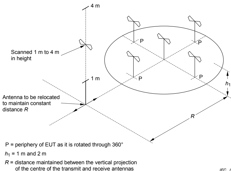
Figure 6b – Typical antenna positions for alternative test site – Horizontal polarization NSA measurements
